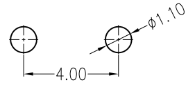
SUGGESTED PCB LAYOUT (COMPONENT SIDE)
